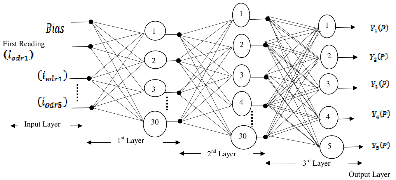
Figure 9: ANN Structure (7-30-30-5) for 5-Wire loops
