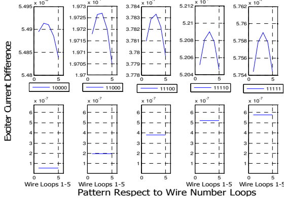
Figure 7: Pattern changes with Fixed Defect Value for 5-Loops Case with Increased Defect at Each Loop with movement exciter scan with 75Hz
