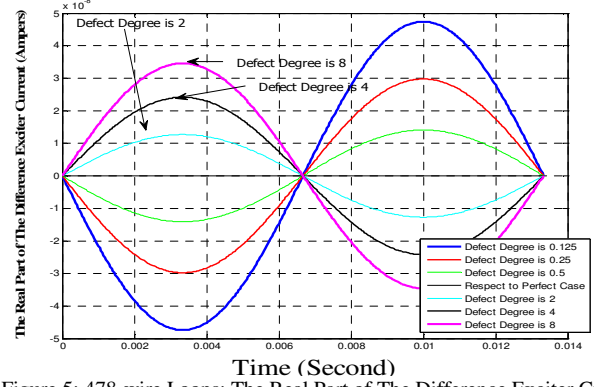
Figure 5: 478-wire Loops: The Real Part of The Difference Exciter Current with Different Defect Values Degrees with Exciter at loop 1 with frequency of 75Hz.
