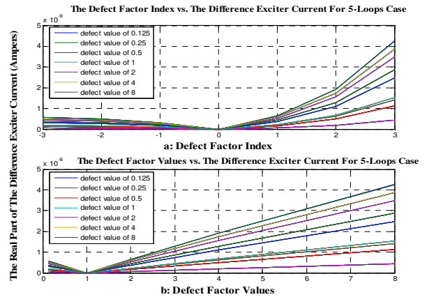
Figure 6: Linear and nonlinear Relationship for The Difference Exciter Current
