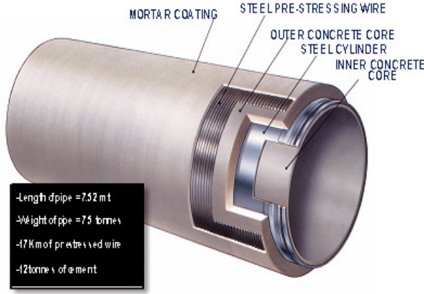
Figure 3: PCCP Material Components
