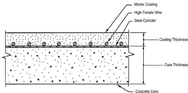
Figure 2[3]: The cross section and elements of Embedded Cylinder Pipe (ECP)
