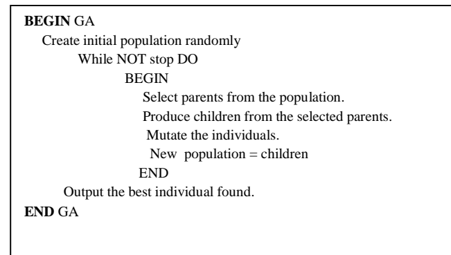
Fig. 2 Abstract Genetic
