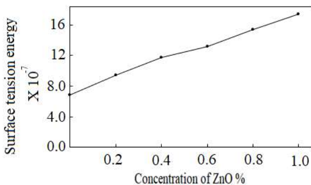
Figure.11. Surface tension energy vs. different concentration of ZnO nanoparticles for PVA/ ZnO nanoparticles solutions at 30°C.
