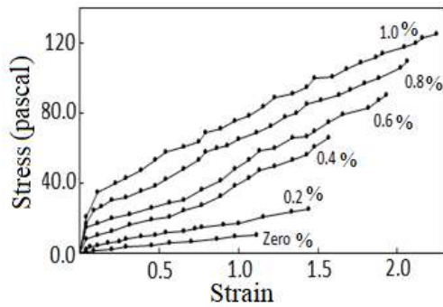
Fig2: The effect of concentration of ZnO nanoparticles on stress-strain curves for PVA/ ZnO nanoparticles thin films.
