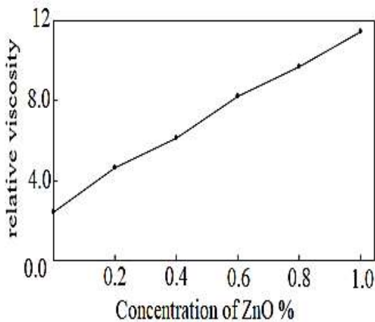
Figure.6. Relative viscosity vs different concentration of ZnO nanoparticles for PVA/ ZnO nanoparticles solutions at 30°C
