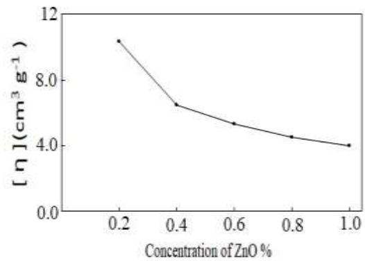
Figure. 8. Intrinsic viscosity vs different concentrations of ZnO nanoparticles for PVA/ ZnO nanoparticles solutions at 30°C.
