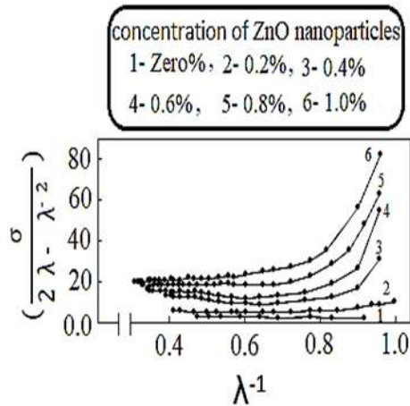
Figure.5. Strain amplification factor curve for PVA/ ZnO nanoparticles thin films.
