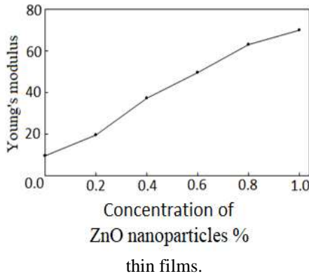
Fig.3. Young's modulus curve of PVA/ ZnO nanoparticles
