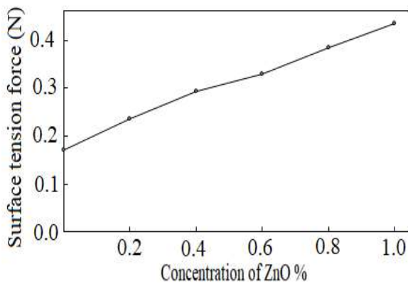
Figure. 10. Surface tension force vs. different concentration of ZnO nanoparticles for PVA/ ZnO nanoparticles solutions at 30°C
