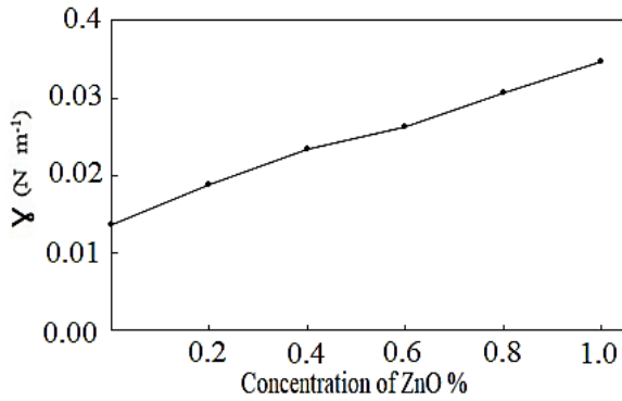
Figure.9. Surface tension vs. different concentrations of ZnO nanoparticles for PVA/ ZnO nanoparticles solutions at 30°C.
