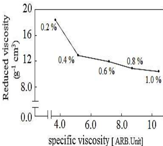
Figure. 7. Reduced viscosity vs specific viscosity nanoparticles for PVA/ ZnO nanoparticles solutions with different concentration of ZnO nanoparticles at 30°C
