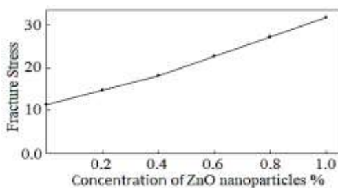
Fig. 4: Fracture stress curve of PVA/ ZnO nanoparticles thin films.
